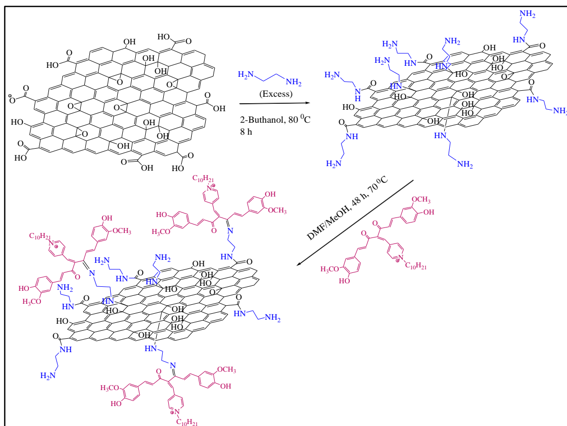
Fig. 1. Synthesis of GN-CP nanohybrid.
