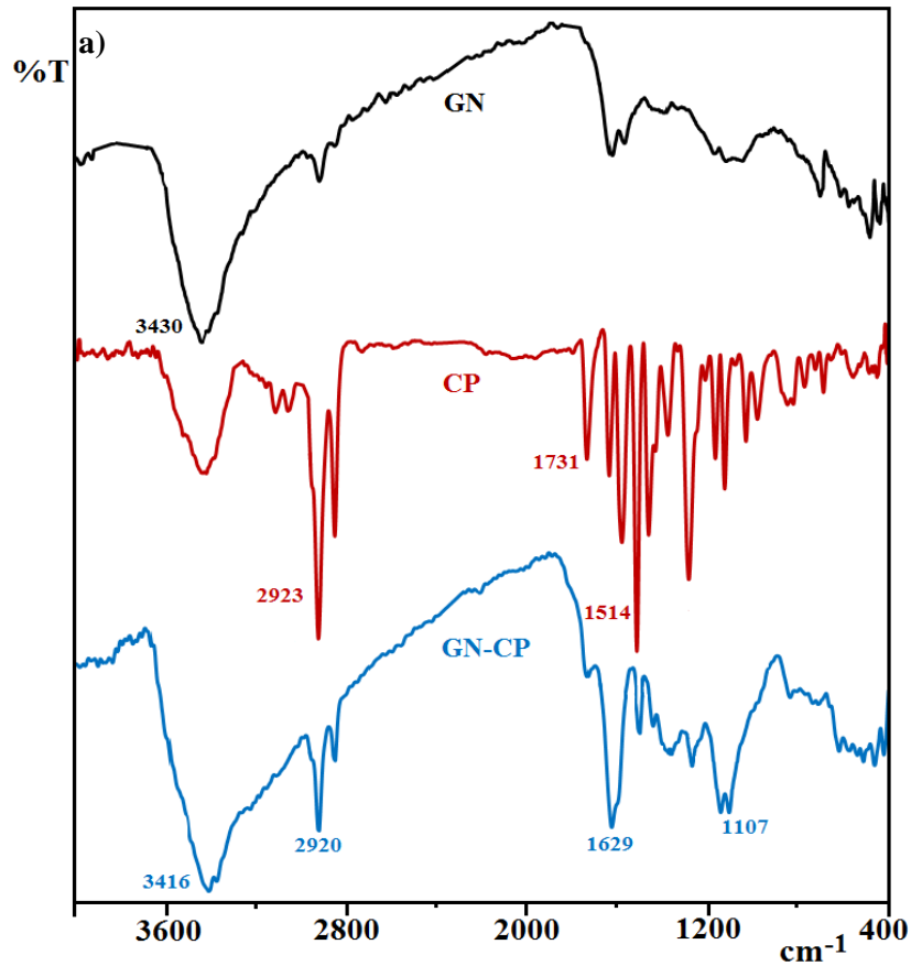
Fig. 2. FT-IR spectra of GN, CP and GN-CP.
